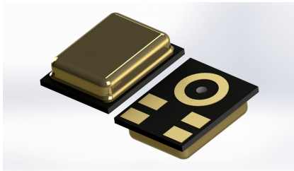
RHLGA metal cap 5-lead 3.5 x 2.65 x 0.98 mm
